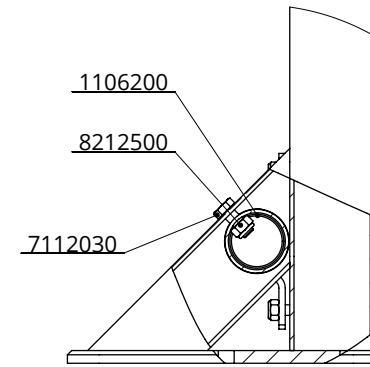
detail C (1 : 5)
